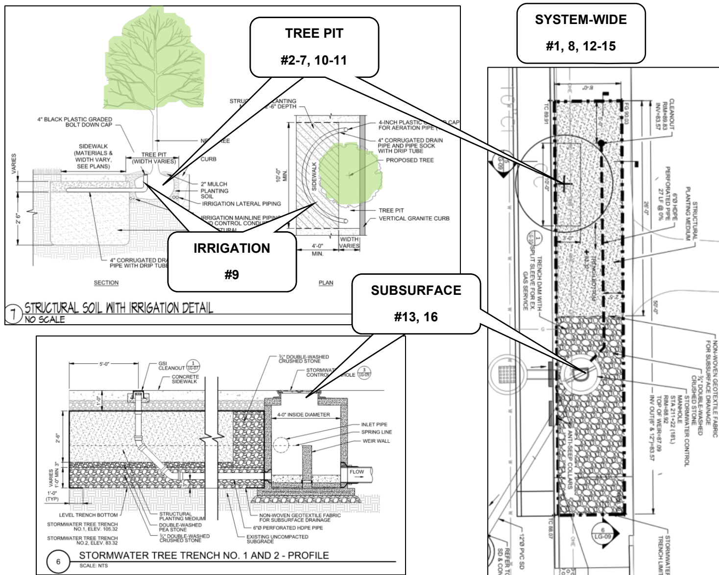
Stormwater Tree Trench – Example Maintenance Figure
