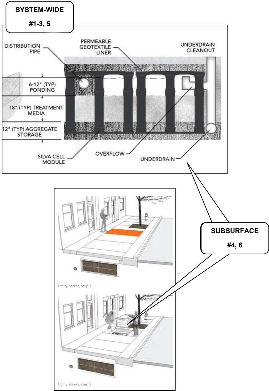
Modular Storage Unit (i.e., Silva Cell) – Example Maintenance Figure
